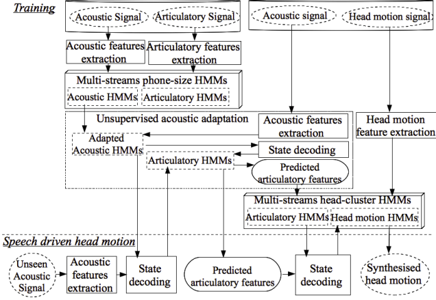
Figure 1: Overview of the speech driven head motion synthesis system.
